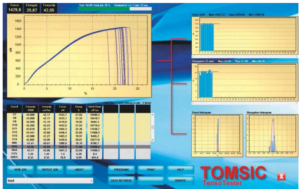
TensoTester3 software.
